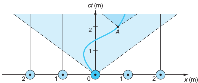
FIGURE 1-21 The speed-of-light limit to the speeds of particles limits the slopes of worldlines for particles that move through x=0 at ct=0 to the shaded area of spacetime, that is, to slopes < -1 and > +1 . The dashed lines are worldlines of light flashes moving in the -x and +x directions. The curved worldline of the particle shown has the same limits at every instant. Notice that the particle's speed = 1/\text{slope} .
